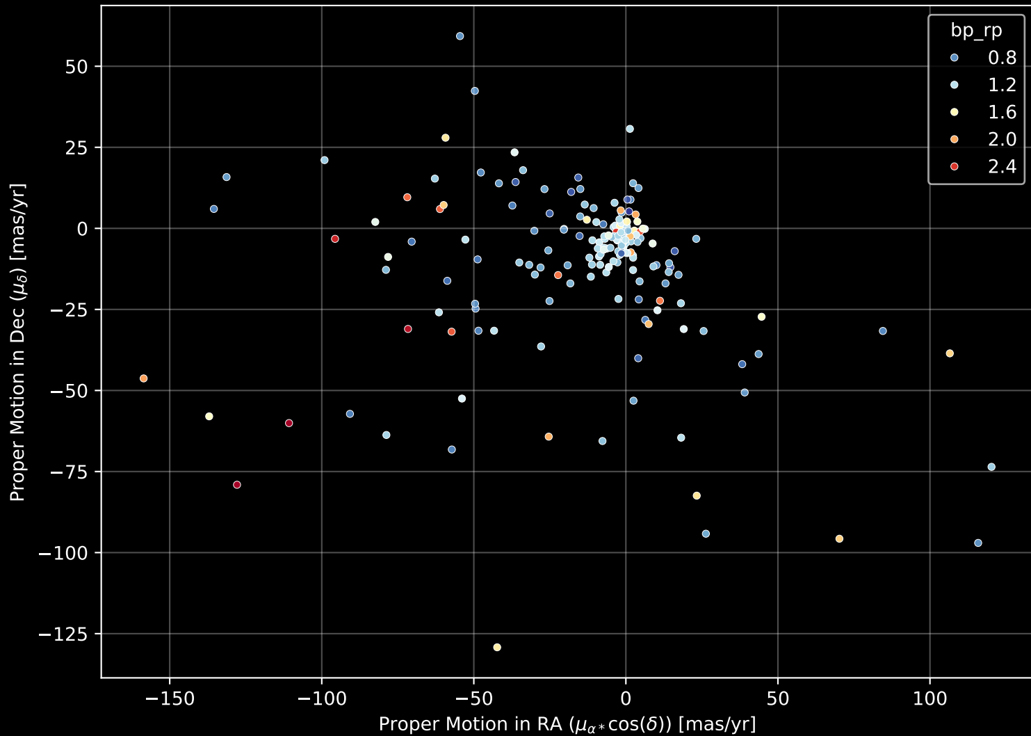
APOGEE DR17 Field: [246+77_btx] Proper Motion Diagram (n= 188)
