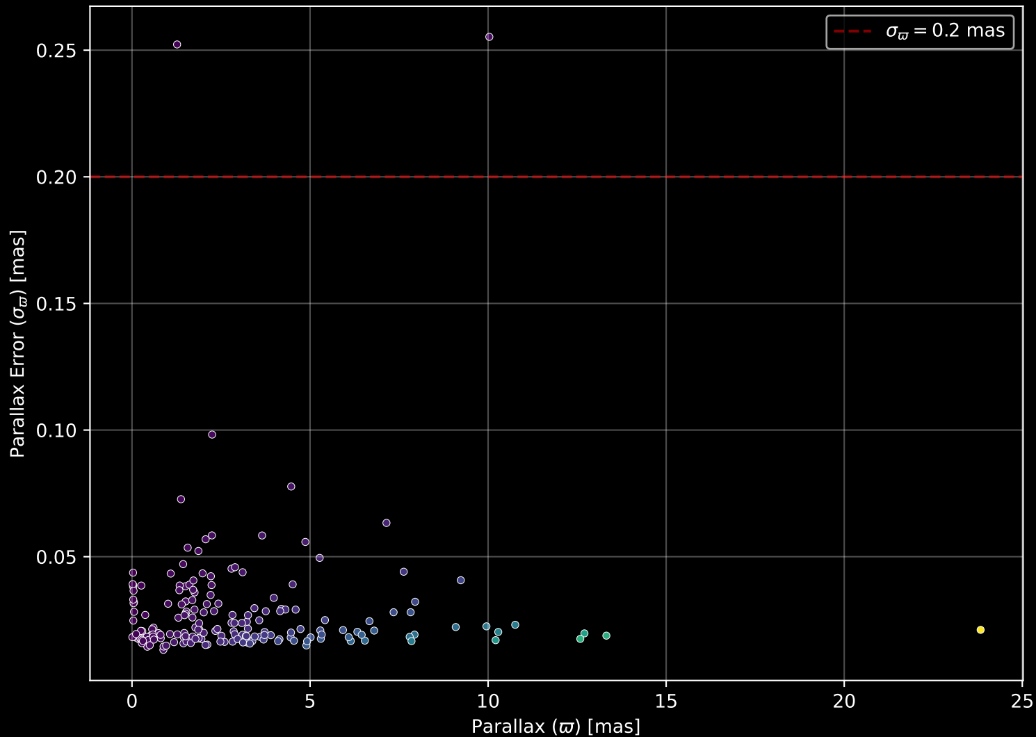
APOGEE DR17 Field: [246+77_btx] Parallax Quality (n= 188)
