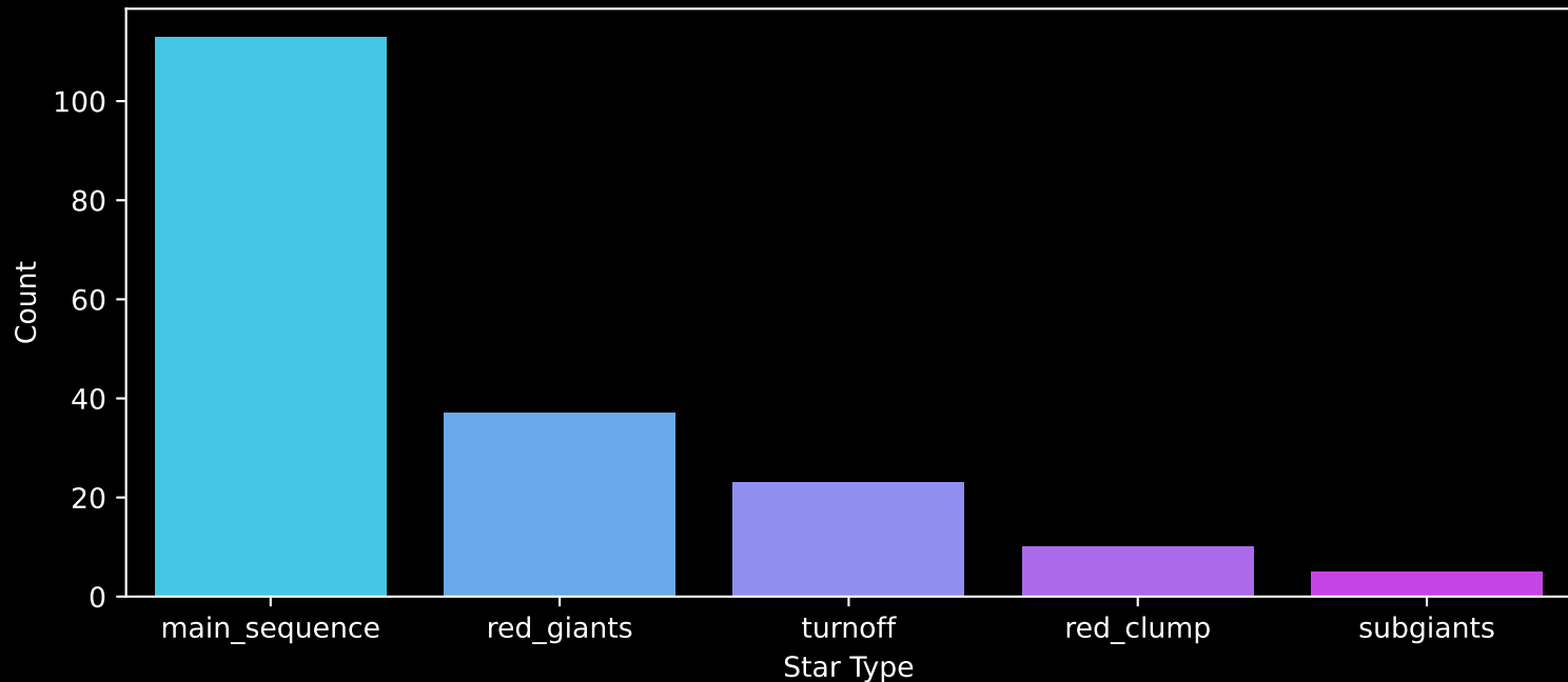
APOGEE DR17 Field: [246+77_btx] Count plot of Star Type
