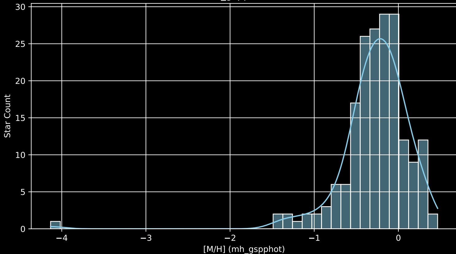
APOGEE DR17 Field: [246+77_btx [M/H] (mh_gspphot) (n= 188)
