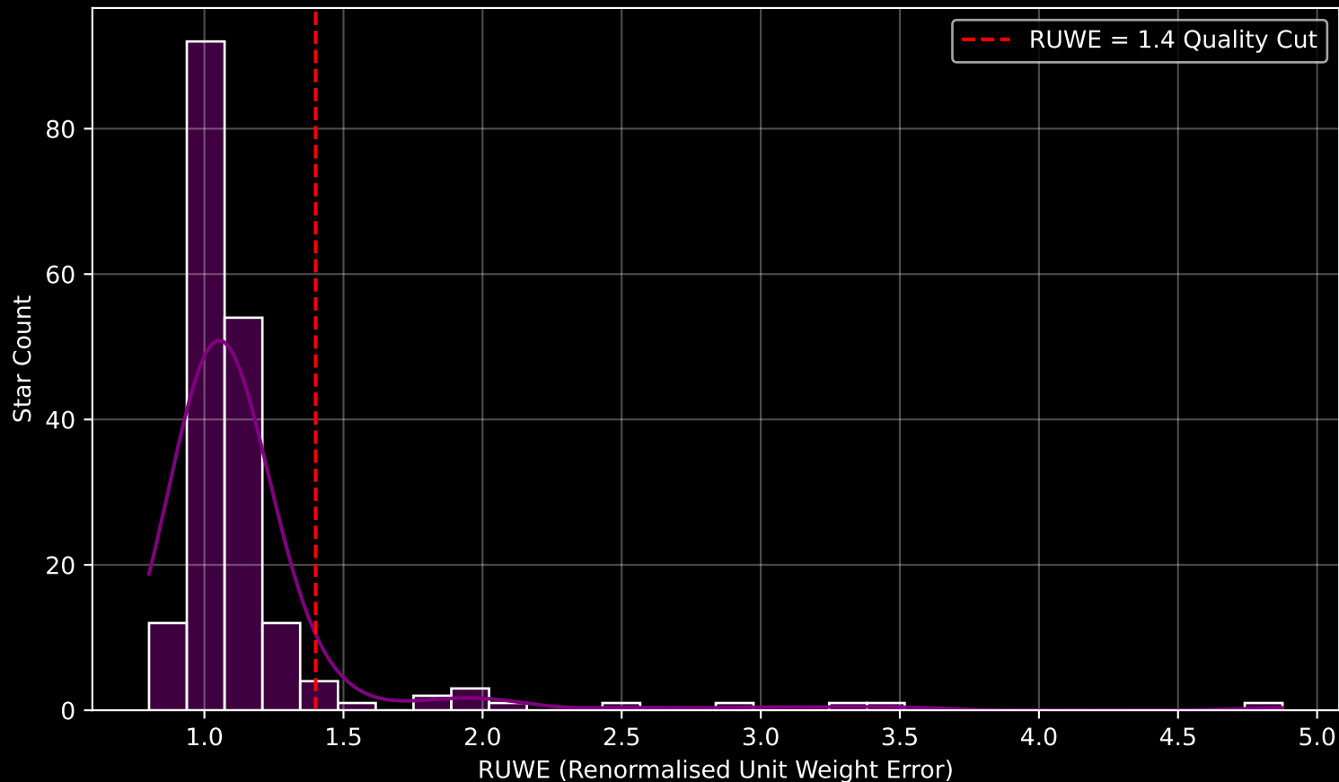
GAPOGEE DR17 Field [246+77_btx] RUWE Distribution (n= 186)
