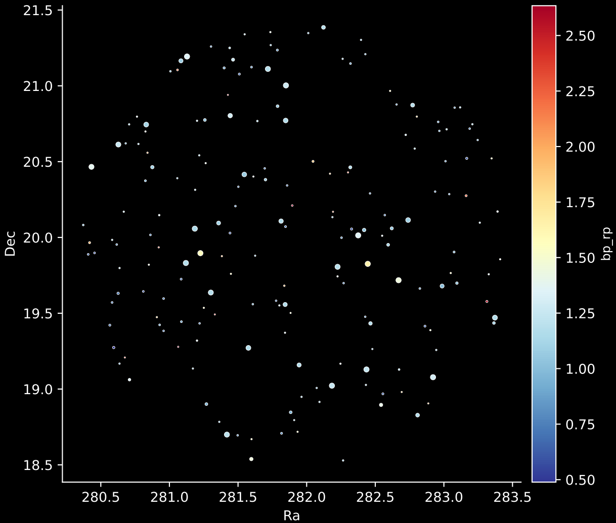
APOGEE DR17 Field: [246+77_btx] Stars: 188
